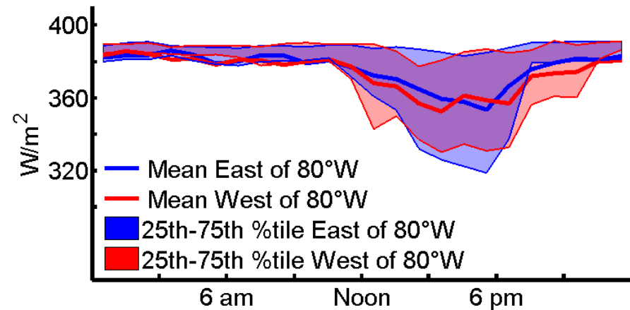
Longwave Radiation
