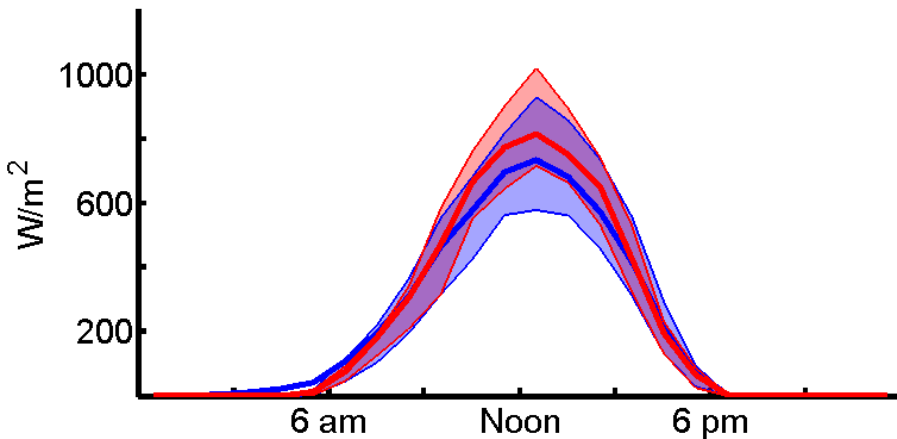
Shortwave Radiation
