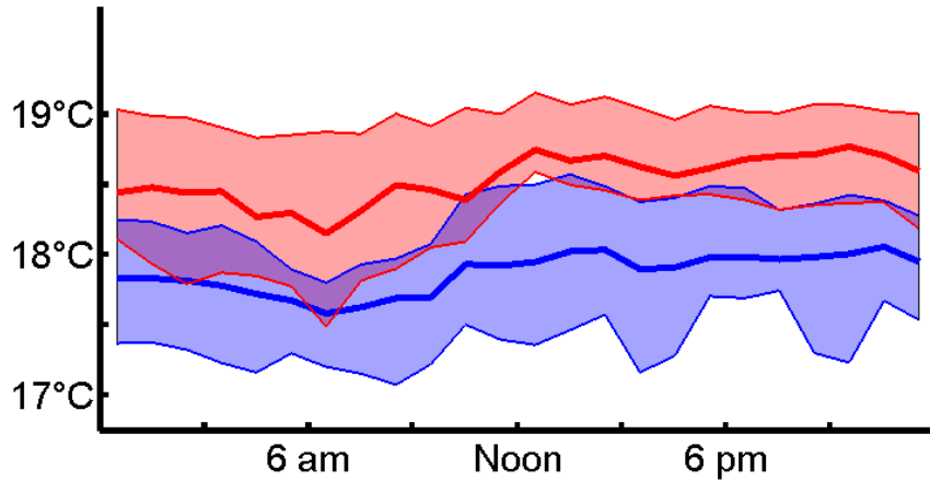
Temperature
