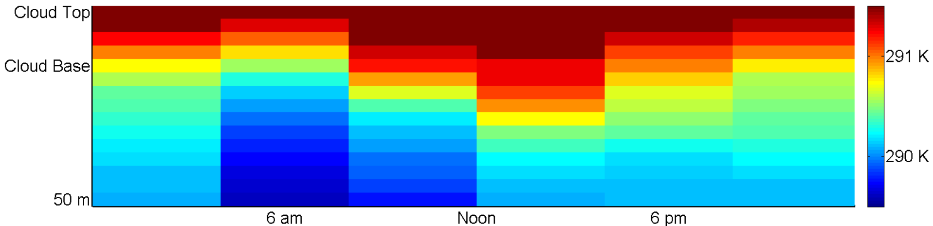
Potential Temperature
